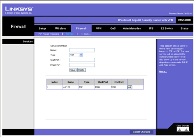
Figure 6-40: Firewall - Services
